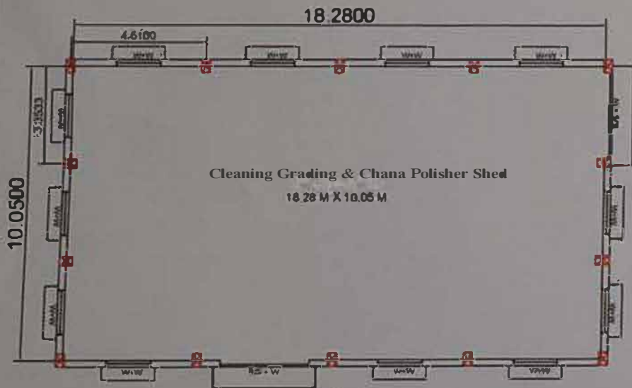
C&G and Chana Polisher Machine SHED scale 1:100 SIZE 18.28 M X 10.05 M X 12.05 M
